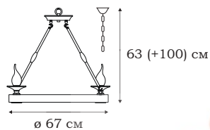
■ L22406.75 6 x LED (3W)
