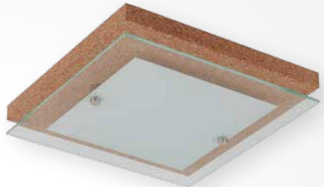
Item no. 4022938 ↔ 290 ↗ 290 ↓ 65 mm incl. 1xLED 14W, 1200lm, 2700K
